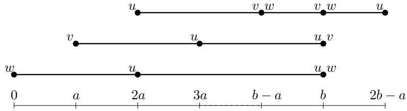
FIGURE 25. \mathfrak{s} -Reduction of the QQD scheme, \mathfrak{s} \in R^5
