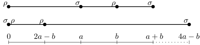
FIGURE 16. s -Reduction for the system (3.19), with \mathbf{s} \in R^3
