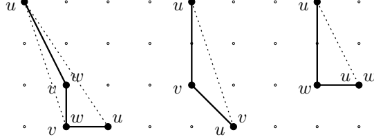
FIGURE 19. Graphical representation of the QQD scheme
