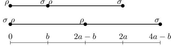
FIGURE 15. s -Reduction for system (3.19), with \mathbf{s} \in R^2
