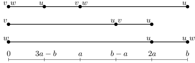
FIGURE 24. \mathfrak{s} -Reduction of the QQD scheme, \mathfrak{s} \in R^4
