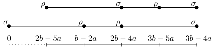
FIGURE 17. s -Reduction for the system (3.19), with \mathbf{s} \in R^4 , b \leq 3a
